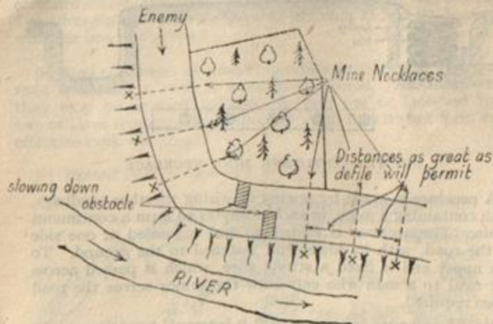
FIG 19.—NECKLACE OR SLED ROAD BLOCK
