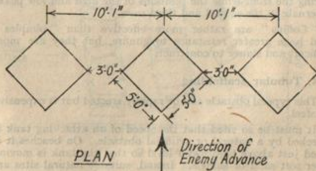
FIG 7.—REINFORCED CONCRETE CUBES
