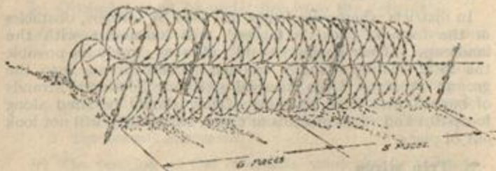
FIG 21.—TRIPLE CONCERTINA FENCE
