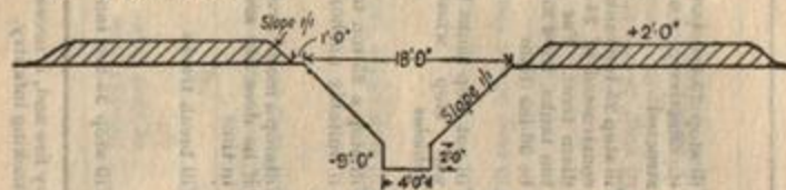
FIG 4.—V TANK DITCH
