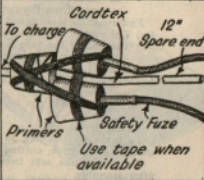
Fig 8. Alternative initiation of cordtex
