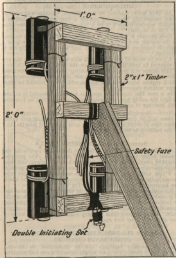
Fig 16. Pole charge for "mouseholing"
