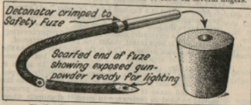
Fig 2. Safety fuzer, No. 27 detonator and 1 oz. primer
